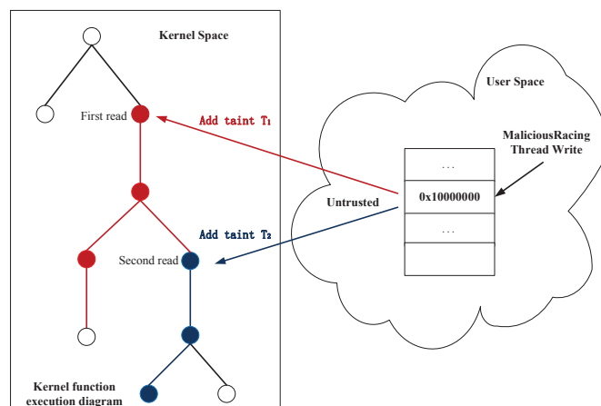
Fig. 6 Multi-taint parallel tracking overview
