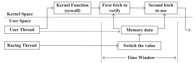
Fig. 1 Illustration of how a double-fetch bug occurs
