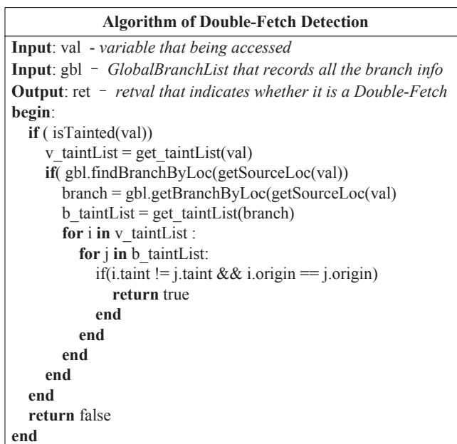
Fig. 10 Algorithm of double-fetch detection
